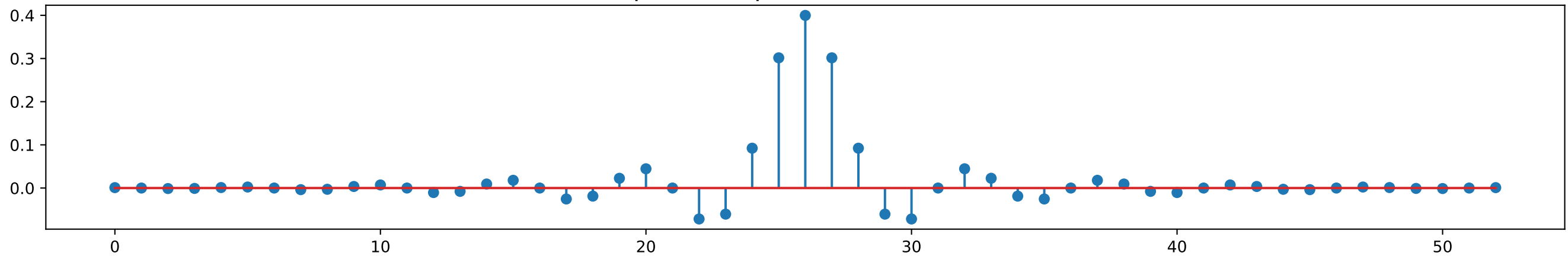
Impulse Response of Filter h2[n]
